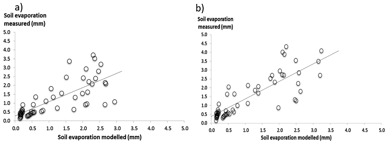
Fig. 10. Soil evaporation measured and modelled in AFS (a) and in FS (b).
