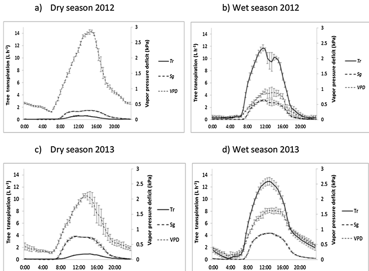
Fig. 7. Typical diurnal patterns of transpiration ( \text{L h}^{-1} ) by Tabebuia rosea (Tr) and Simarouba glauca (Sg) trees and VPD (kPa) from mean of five consecutive days in the 2012 dry (a) and wet seasons (b) and in the 2013 dry (c) and wet seasons (d). Bars represent the standard error of the mean.
