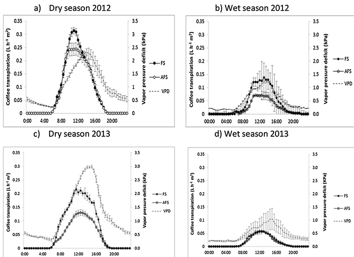
Fig. 4. Typical diurnal trends in coffee transpiration on a leaf area basis from mean of four coffee trees each in FS and AFS over five consecutive days in the 2012 dry (a) and wet season (b) and 2013 dry (c) and wet season (d), compared with VPD. Bars represent the standard error of the mean.
