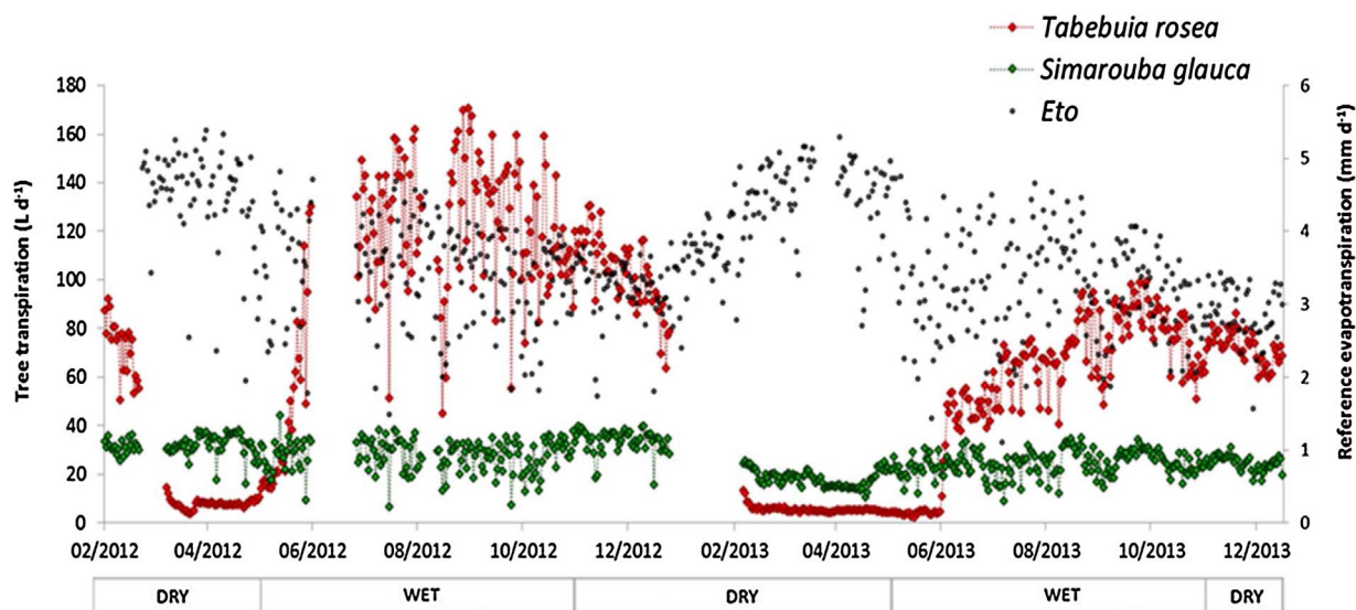
Fig. 6. Transpiration per day in Tabebuia rosea and Simarouba glauca trees, with calculated reference evapotranspiration (ETO).
